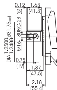
K Parallel with key ISO 3019-1 32-1
