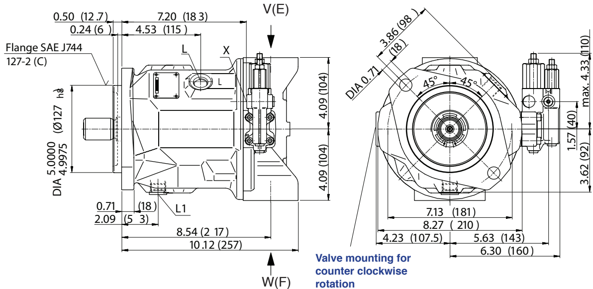
View V Model 92
