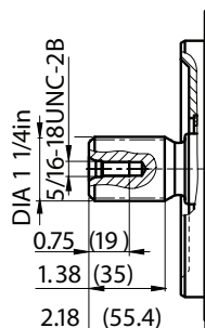
U Splined shaft 1 1/4 in 14T 12/24 DP1) SAE J744 - 32-4 (C) 1)
