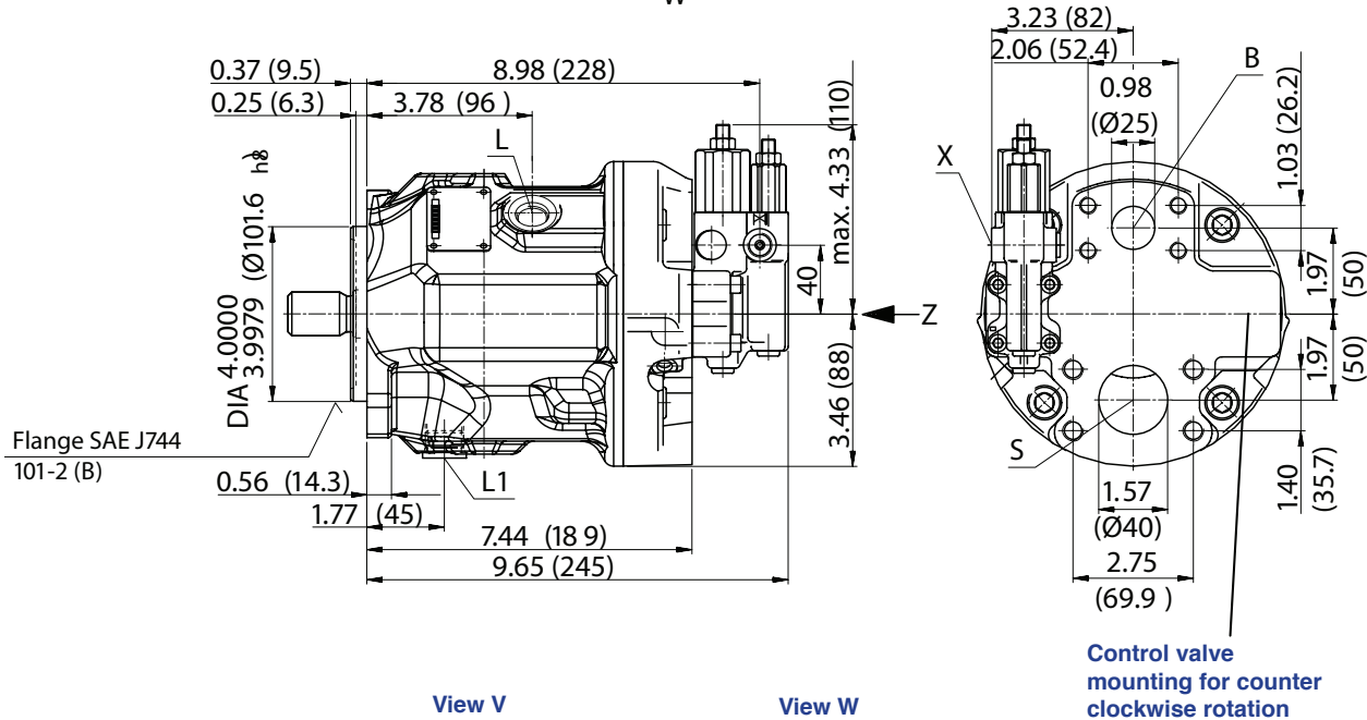
Port Plate 61/11 N00
