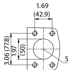
View W Model 92
