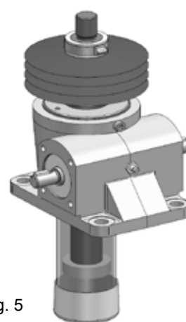
Screw jack with Stop nut SM
