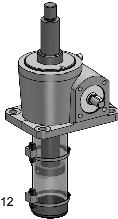
MLS Magnetic Limit switches
