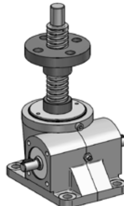
BDL Screw jack with Lifting nut
